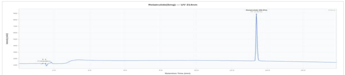
Retatrutide 5mg - RT5-260825-H: UV Chromatogram
