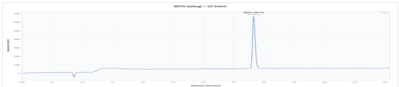
MOTS-C 10mg - MS10-260724-H: UV Chromatogram
