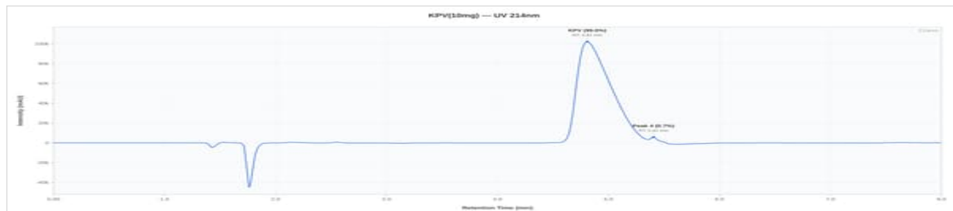
KPV 10mg - KPV10-260627-A: UV Chromatogram
