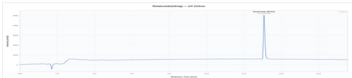
Retatrutide 10mg - RT10-260708-H: UV Chromatogram
