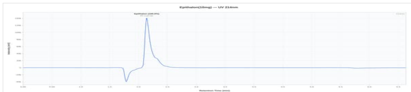
Epitalon 10mg - ET10-260630-BA: UV Chromatogram
